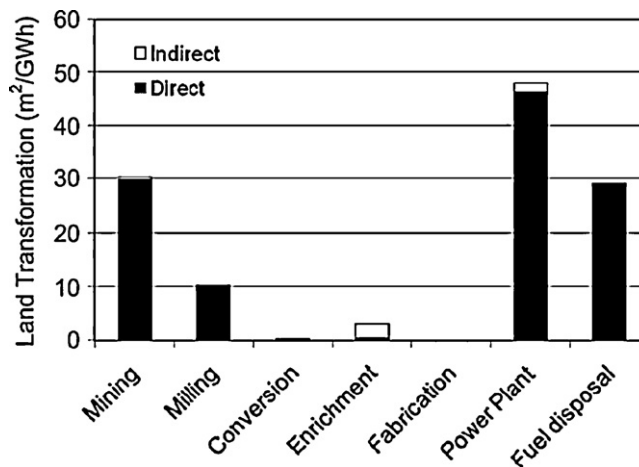
Figure 1: Land Transformation during the Nuclear-Fuel Cycle. Source: Fthenakis and Kim (ref. 17).
